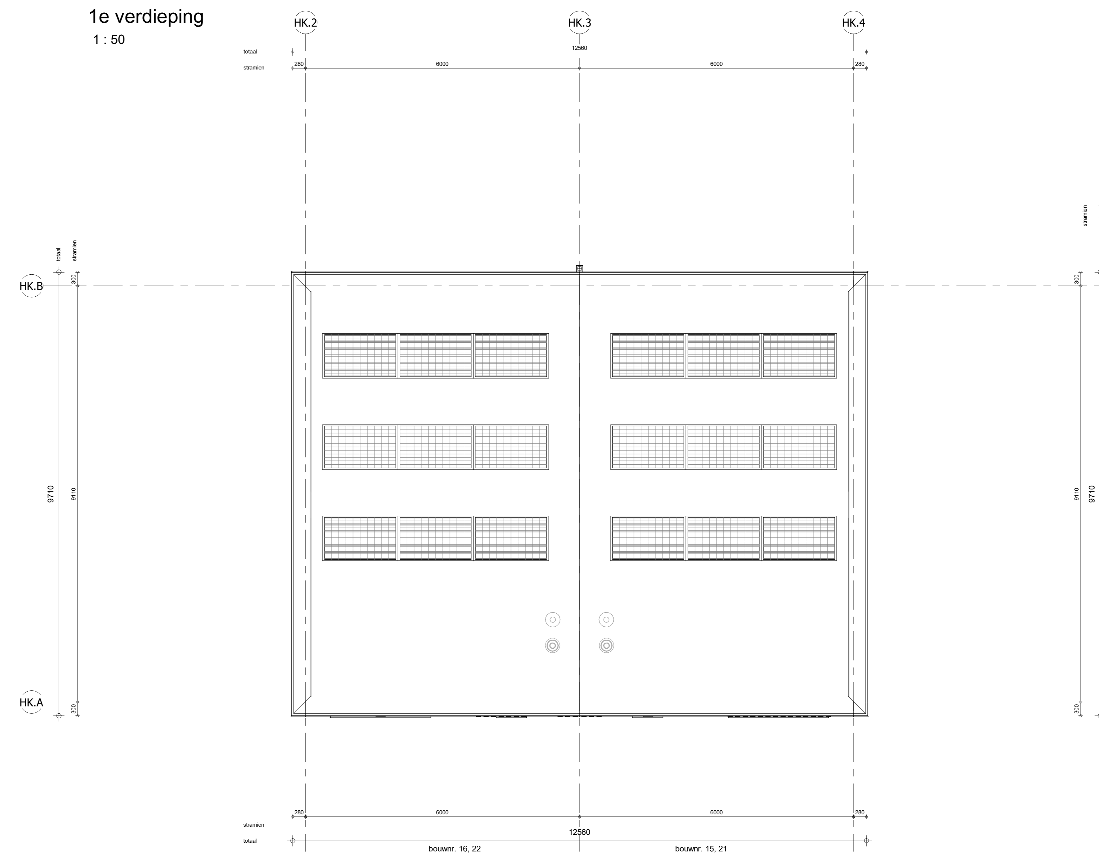
dakplan 1:50
